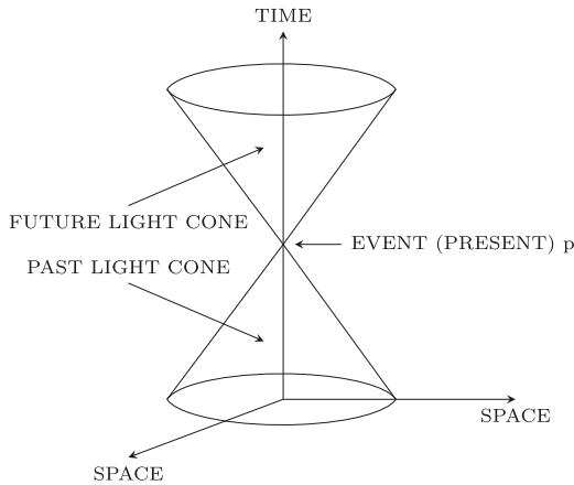
Figure 1: Minkowski diagram representing two light-cones around point p .
