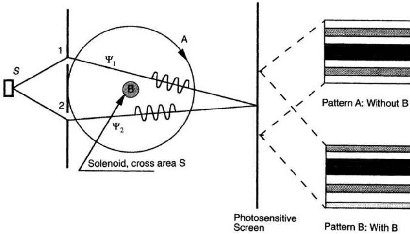
Figure 2: (From Liu 1994, p. 990). \Psi_1 and \Psi_2 represent the paths of electrons from the source S on the left to the screen on the right, and B represents the magnetic field within the solenoid. When field B is present, the interference pattern on the screen shifts from pattern A (above) to pattern B (below).
